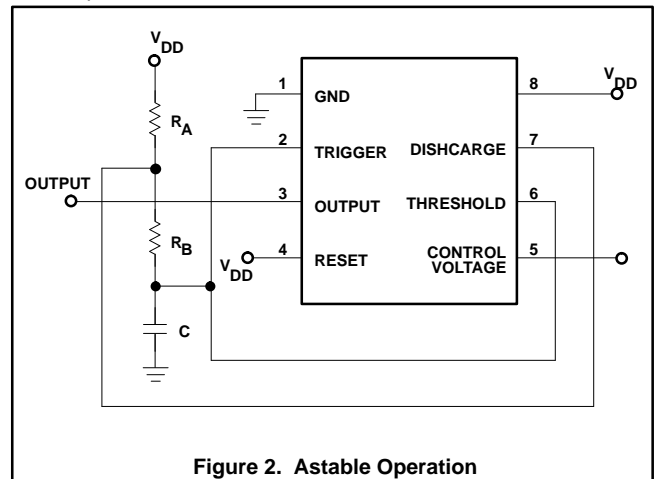
Figure 2. Astable Operation
