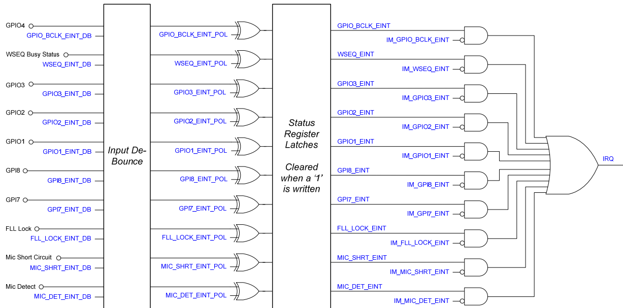
Figure 60 Interrupt Controller
