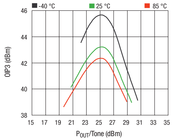
OIP3 vs. P_{OUT}/\text{Tone} Across Temperature
