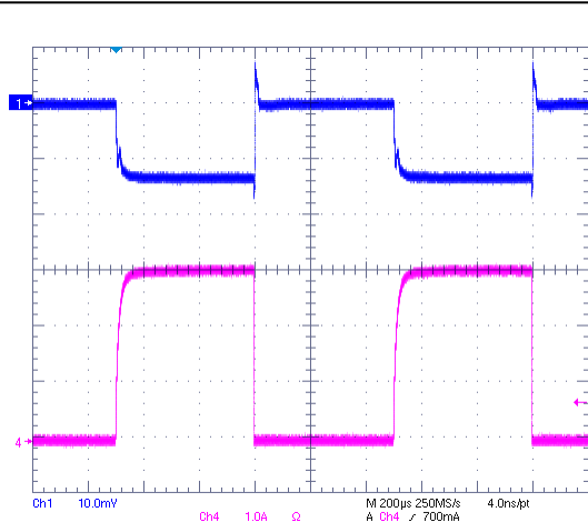
VIN=2.5V, VCNTL=5V, VOUT=1.25V @ 3A Sourcing
