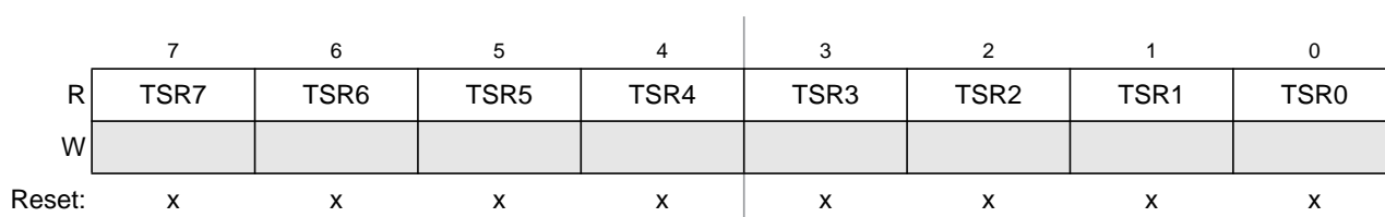
Figure 10-38. Time Stamp Register — Low Byte (TSRL)
