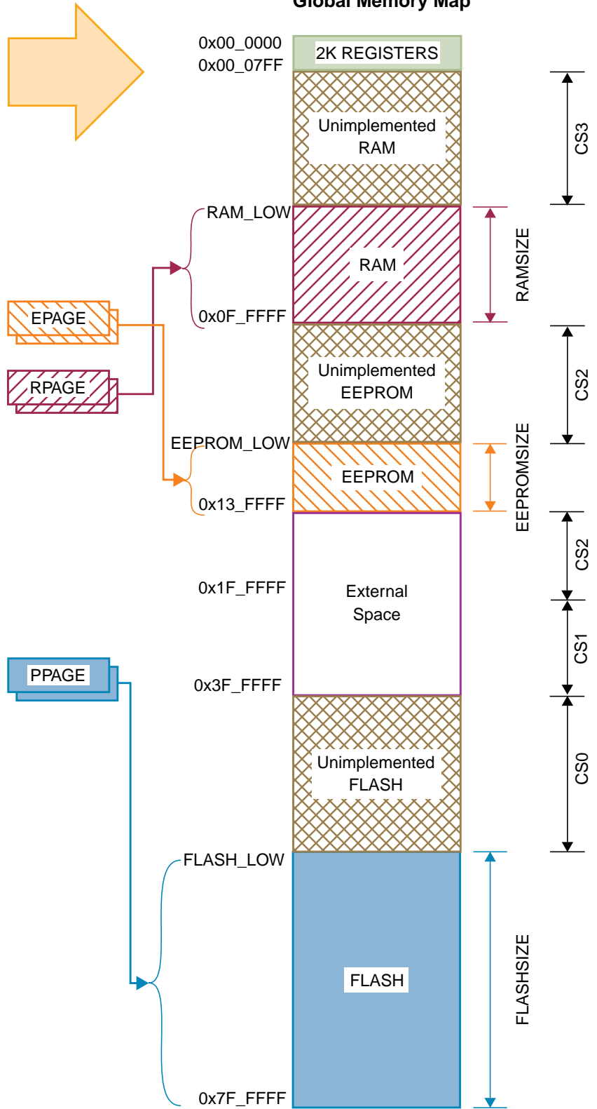
Figure 1-3. S12X CPU & BDM Global Address Mapping
