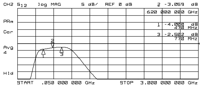
S 21 , S 12
