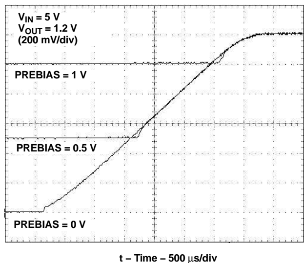
Figure 21. Startup Waveforms
