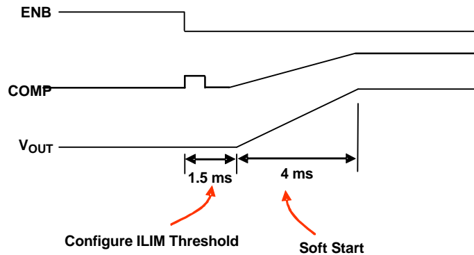
Figure 19. Startup
