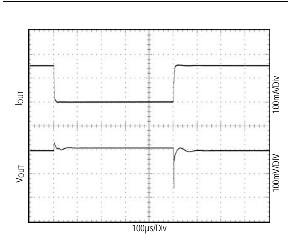
Figure 40. Load Transient; I_{OUT}= 0mA to 150mA V_{IN}=2.0V , V_{OUT}=1.5V
