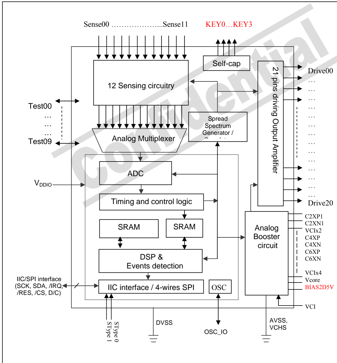
Figure 4-1: SSD2531 Block Diagram
