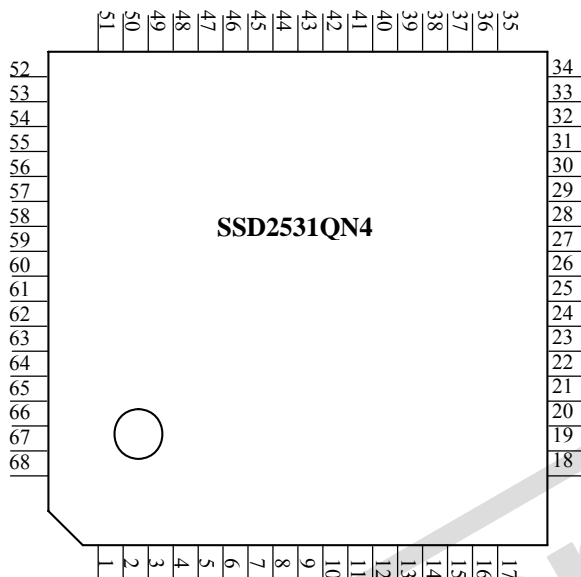
Figure 5-1: Pinout Diagram –68 pin QFN (Topview)
