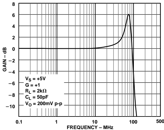
Figure 37. AD8051/AD8052 Closed-Loop Frequency Response: C_L = 50pF
