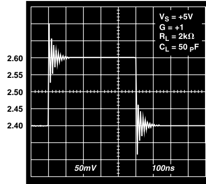
Figure 38. AD8051/AD8052 200 mV Step Response: C_L = 50pF
