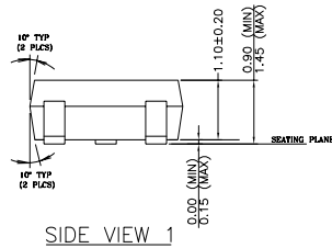
SIDE VIEW 1
