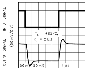
TIME (1 \mu s /DIV) DS011991-66
