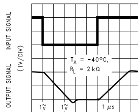
TIME (1 \mu s /DIV) DS011991-67
