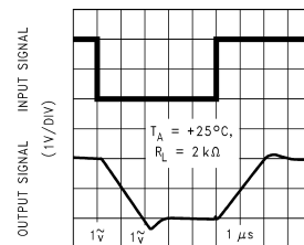
TIME (1 \mu s /DIV) DS011991-68
