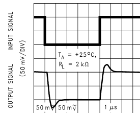
TIME (1 \mu s /DIV) DS011991-65
