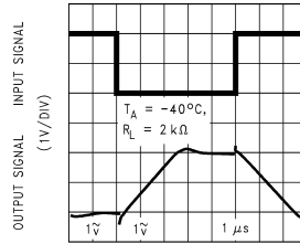
TIME (1 \mu s /DIV) DS011991-61
